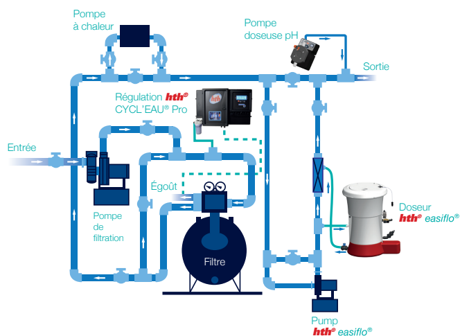
Typical installation diagram for an hth CYCL'EAU® Pro control system with hth easiflo® feeder
